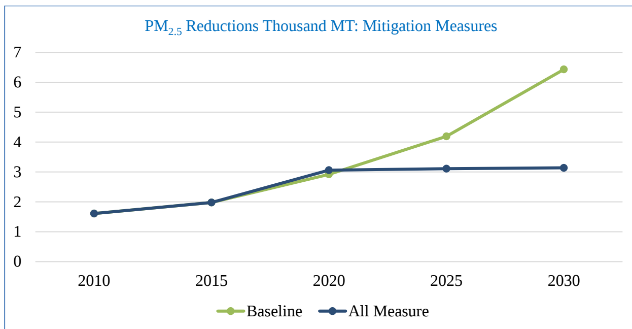
Figure 4.3 PM 2.5 reductions from industry measures
