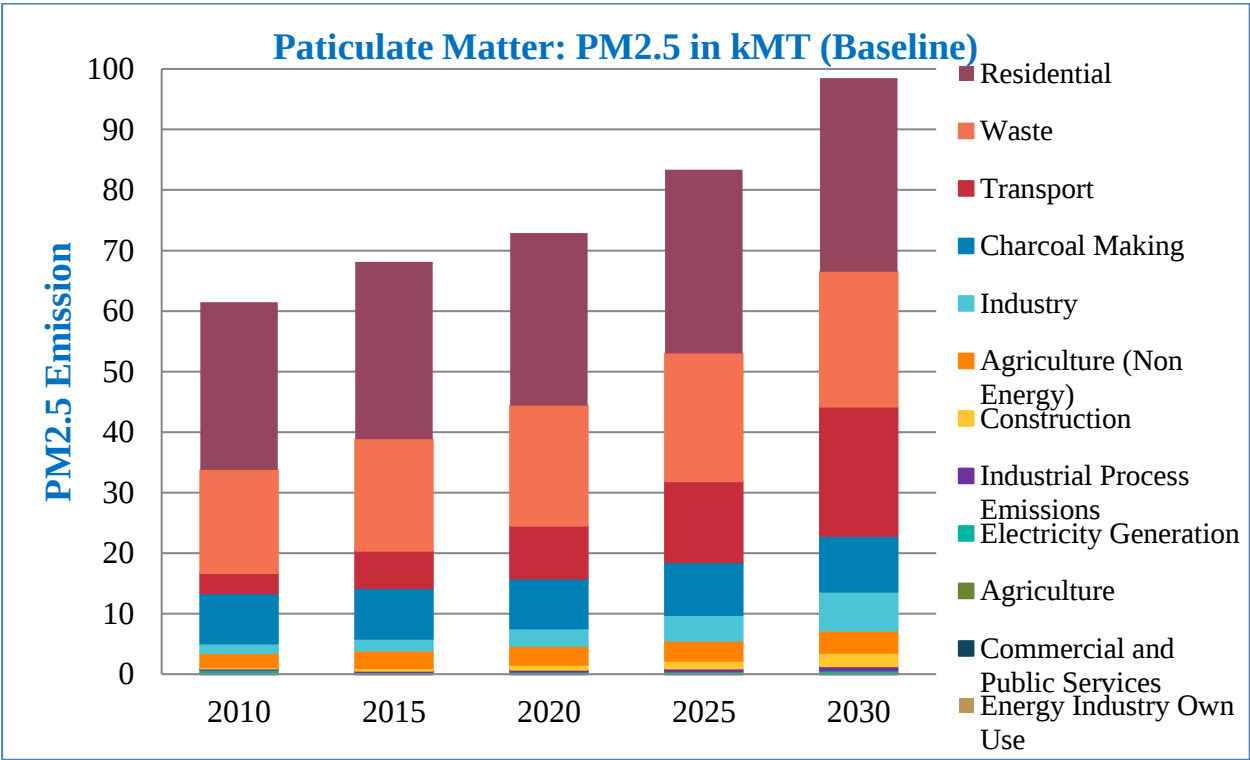
Figure 2.5 Total PM2.5 Emission in Cambodia between 2010 and 2030
