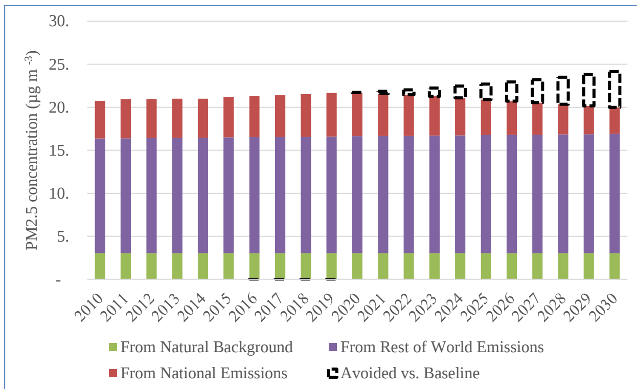
Figure 3.8 Reduction in population-weighted PM 2.5 concentrations for Cambodia from LEAP-IBC for 2010-2030 from the implementation of all measures included in Cambodia's Clean Air Plan, compared to the baseline scenario
