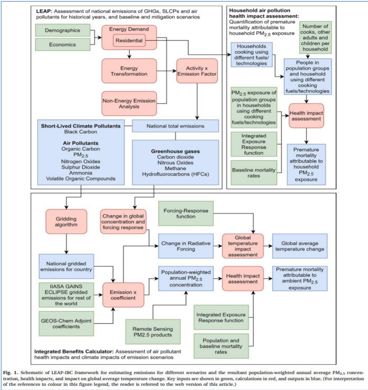
Figure 3.6 Overview of LEAP-IBC calculation framework for air pollution health impact assessment (source: Kuylenstierna et al. 2020).
