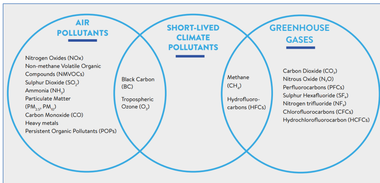
Figure 2.3 Summary of pollutants that are classified as air pollutants, short-lived climate pollutants and greenhouse gases (Source: CCAC SNAP, 2019)
