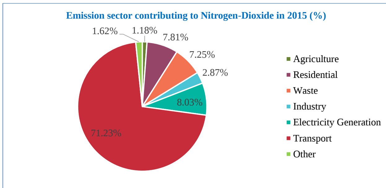
Figure 2.8 Share of Nitrogen Dioxide emission by sector in 2015
