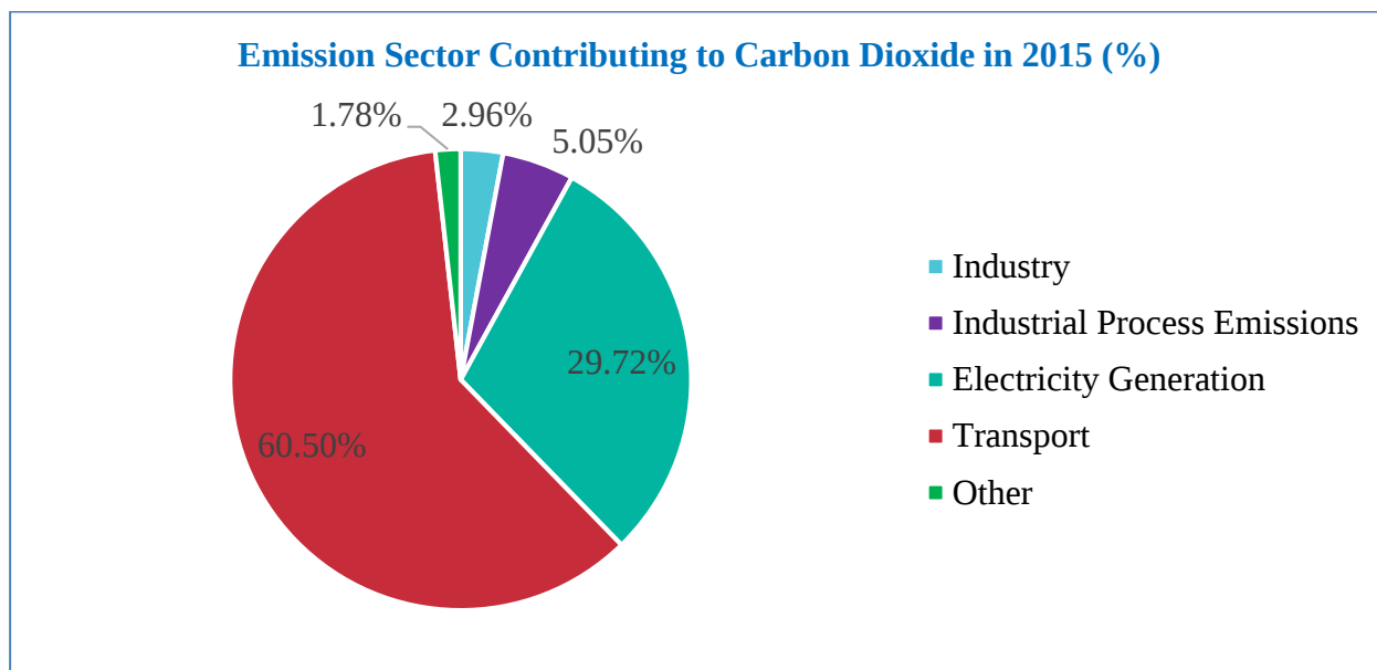
Figure 2.20 Share of Carbon Dioxide emission by sector in 2015
