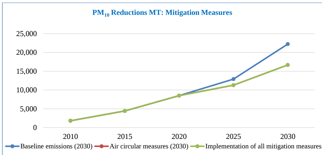
Figure 4.11 PM 10 reductions from construction measures
