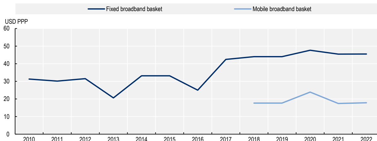
Figure 4.4. Prices for entry-level fixed and mobile communication services, USD PPP, 2010-22
